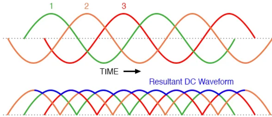
Three-phase AC and 3-phase full-wave rectifier output.
